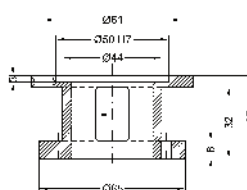
RS15-xx (int. Ø as specified in description)
