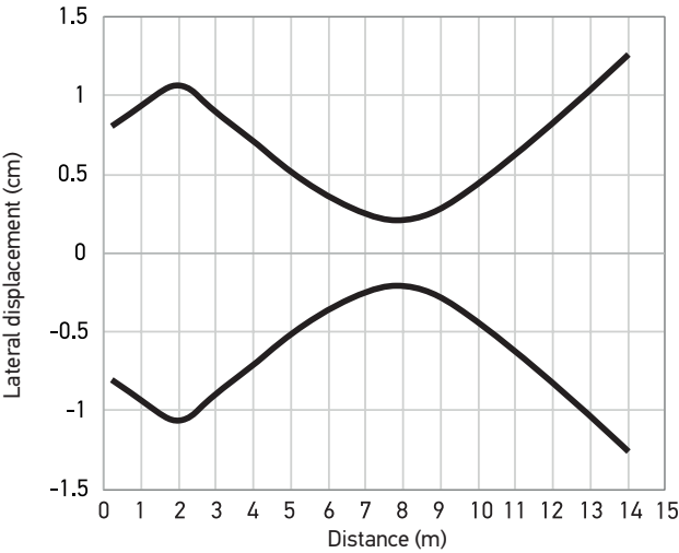
S3N-PH-*-B**-* (Beam diagram)
