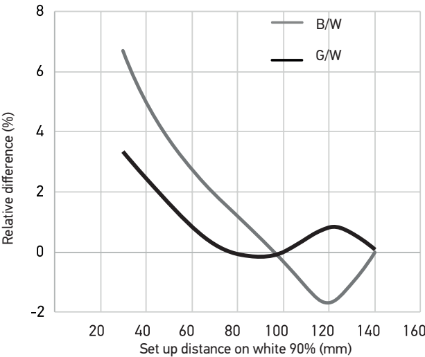
S3N-PH-*-M03-* (Black and white difference)
