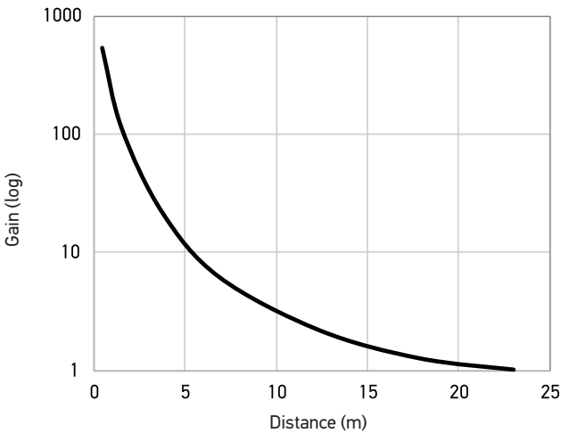
S3N-PR-*-FG**-* (Excess gain)
