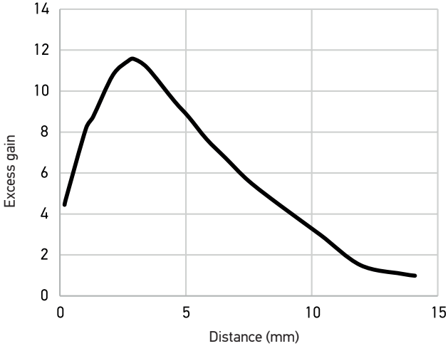
S3N-PH-*-B**-* (Excess gain)
