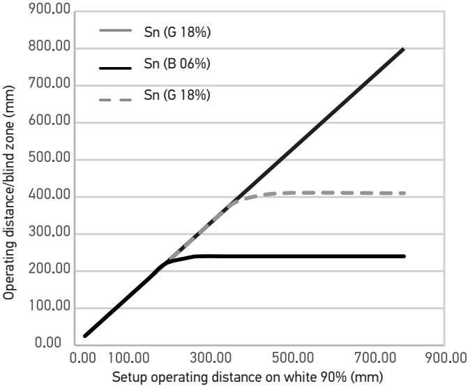
S3N-PR-*-M01-* (Operating distance)
