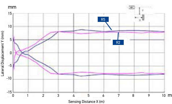
POLARIZED RETROREFLECTIVE - DETECTION AREA
