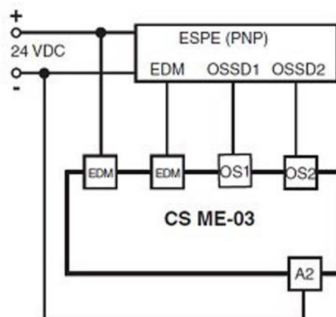
Fig 103 - EDM Relay
