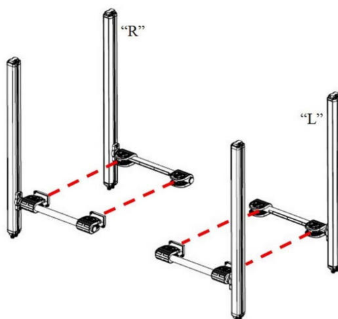
Fig 115 - L-MUTING
