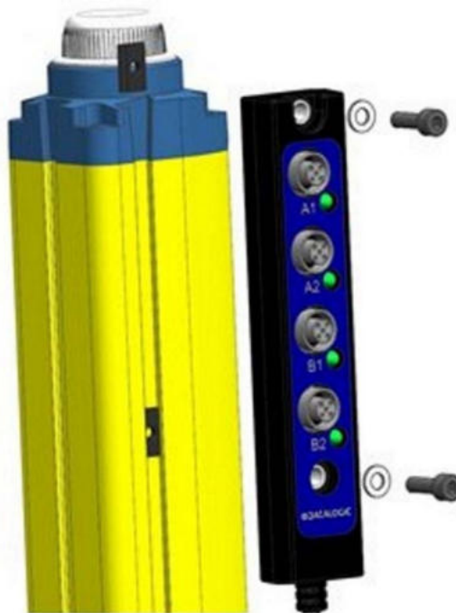
Fig 121 - Connection box
