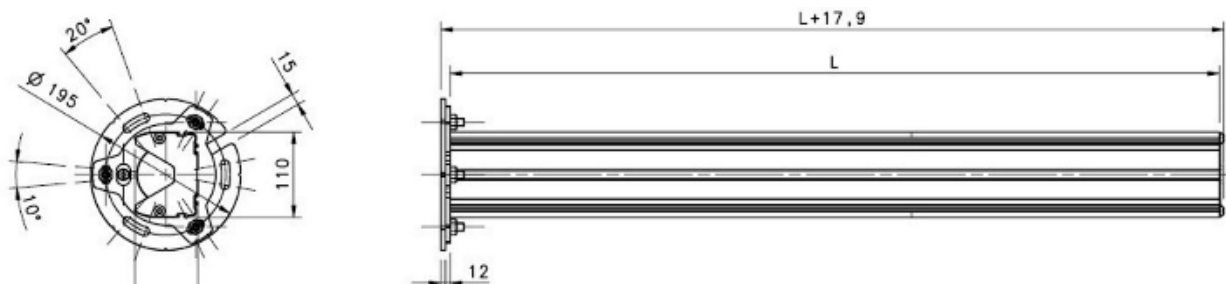
Fig 89 - Dimensions (mm)
