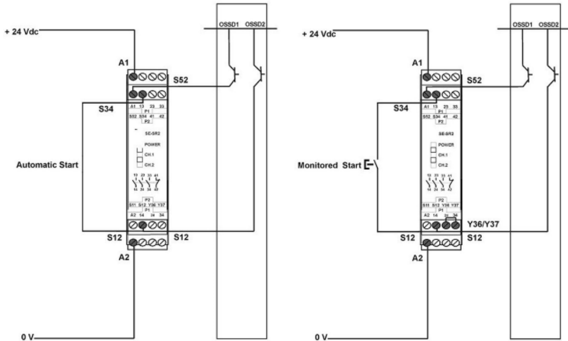
Fig 102 - Safety relay
