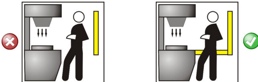
Fig 11 - Wrong light curtain positioning
