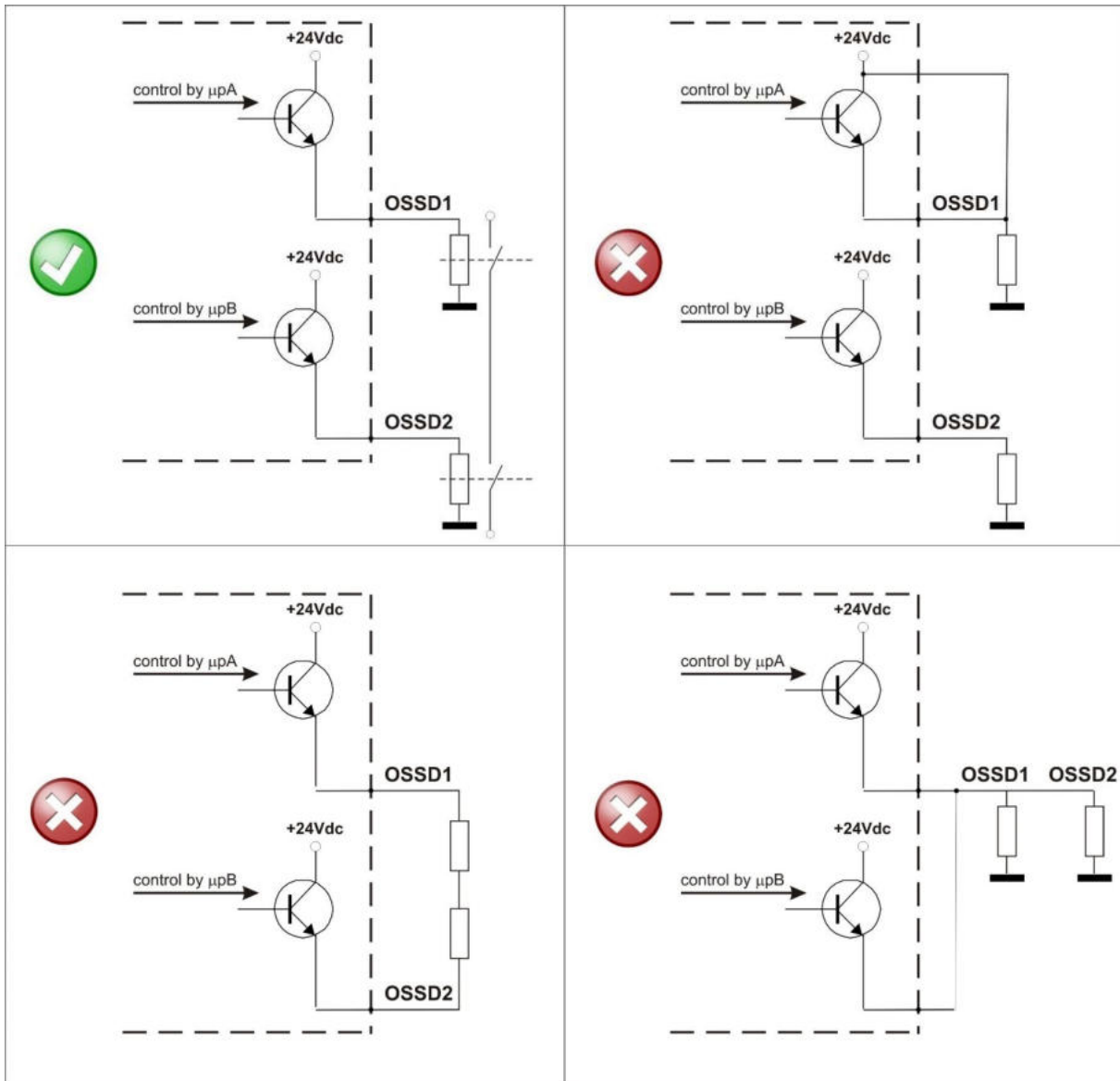
Fig 32 - OSSDs connection
