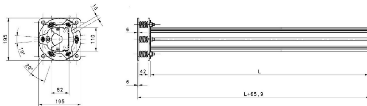
Fig 92 - Mounting
