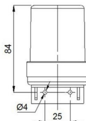
Fig 105 - Lamp LMS-2
