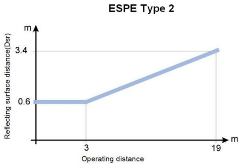
Fig 14 - Minimum distance from reflective surface
