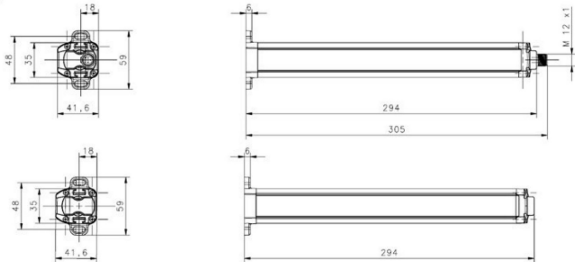
Fig 109 - Dimensions (mm)
