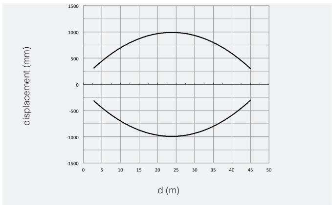
MVE/**-**- MVD/**-**- parallel displacement
