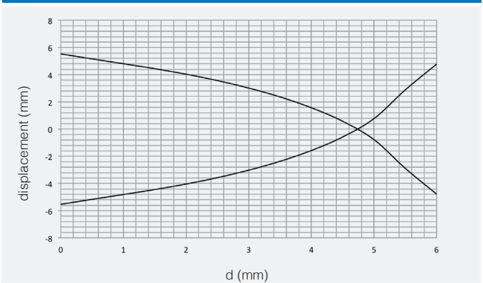
V3K1/**-3* parallel displacement
