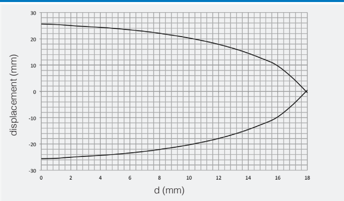
V3T1/**-4* parallel displacement
