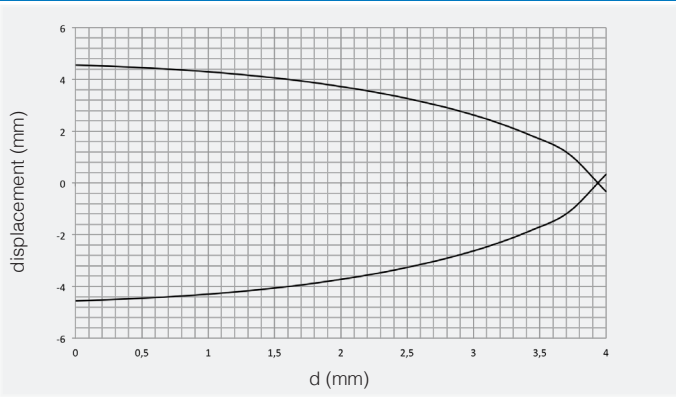
V3M1/**-4* parallel displacement
