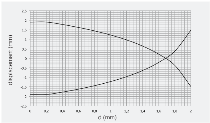
V3M1/**-3* parallel displacement
