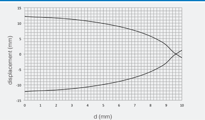
V3K1/**-4* parallel displacement
