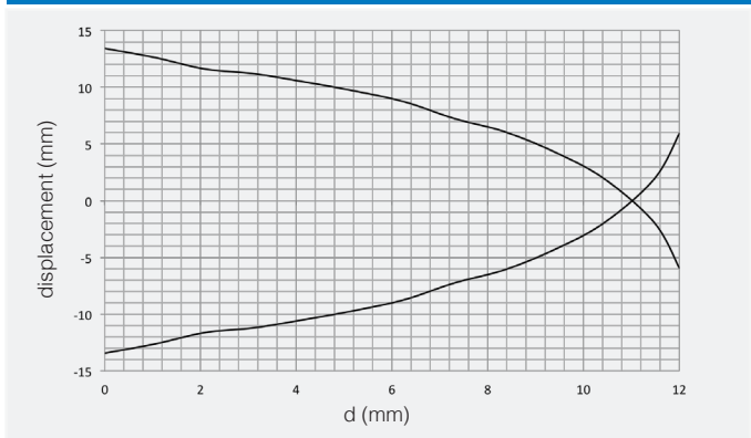
V3T1/**-3* parallel displacement
