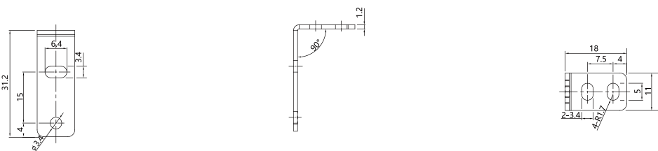
ZJP-13 (PST Mounting rack)
