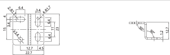
ZJP-13 (PST Mounting rack)
