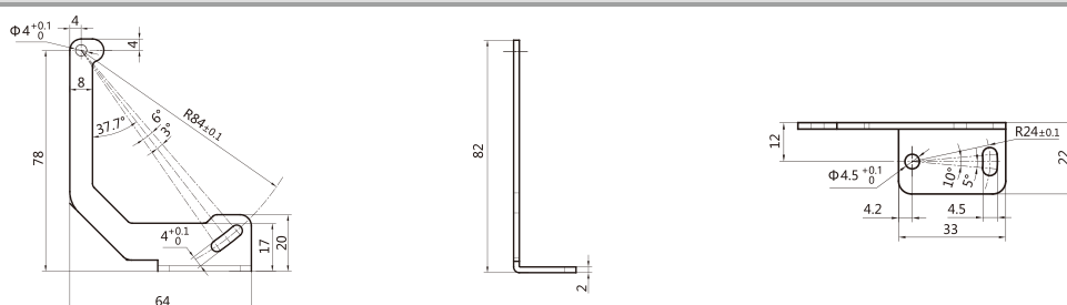
ZJP-7 ( PTB Mounting rack )
