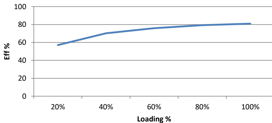
AM1S-1215SZ Efficiency vs. Loading
