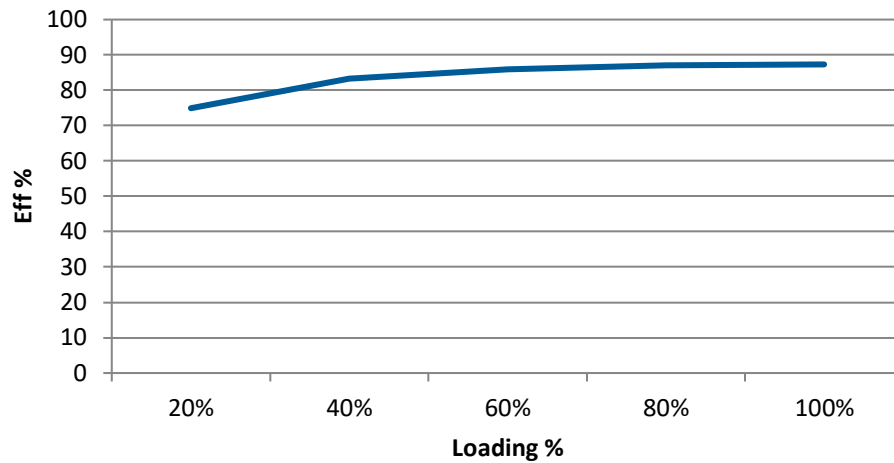
AM3D-0509SZ Efficiency vs. Loading
