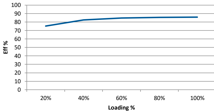
AM3D-1205SZ Efficiency vs. Loading
