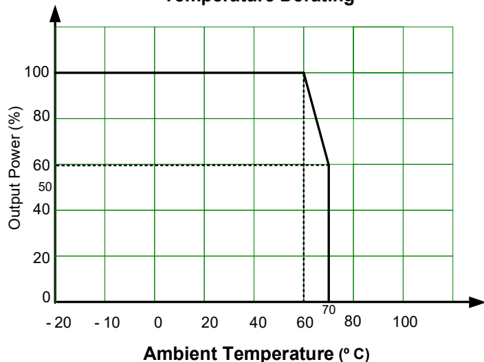
Temperature Derating
