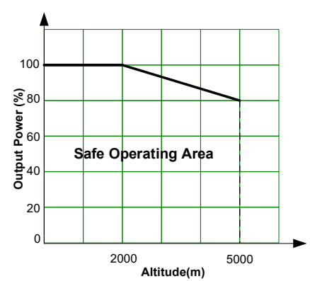
Altitude derating for all models
