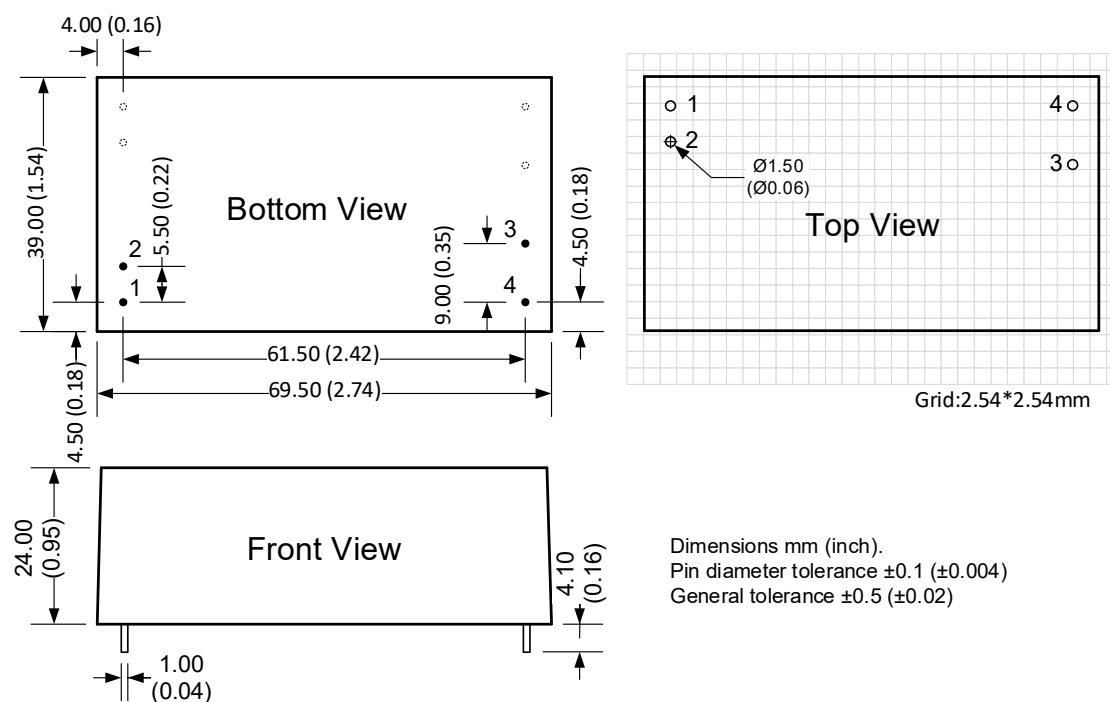
Pin Output Specifications
