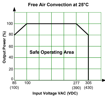
Input derating
