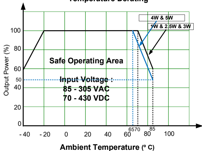
Temperature Derating
