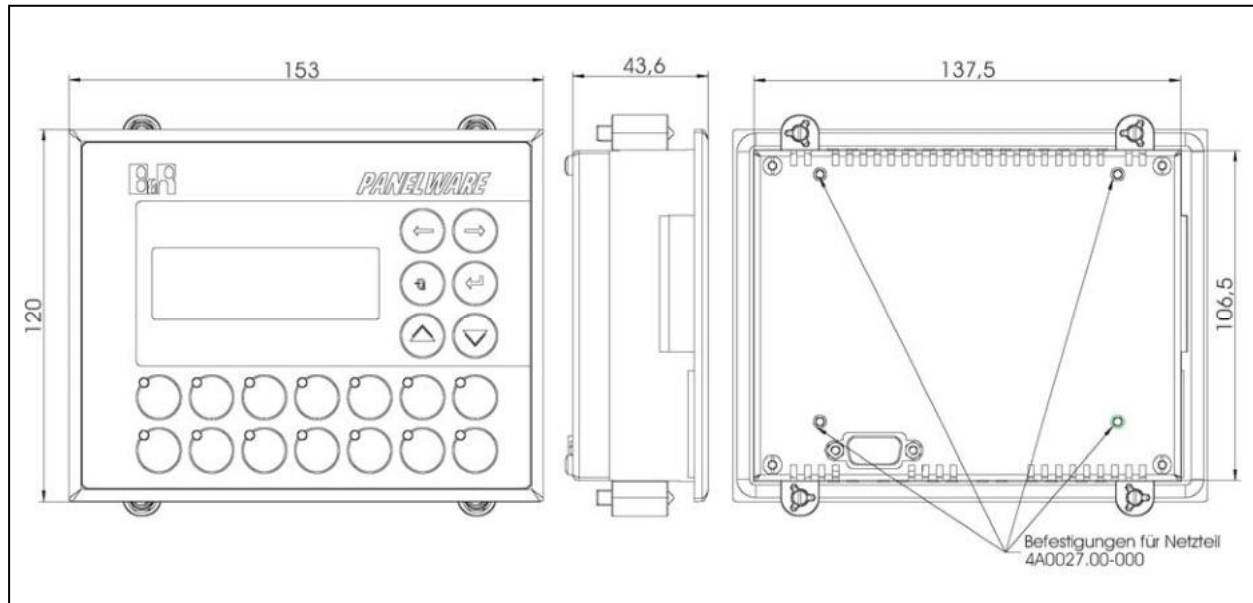
Figure 5: Dimensions - 4B1260.00-390
