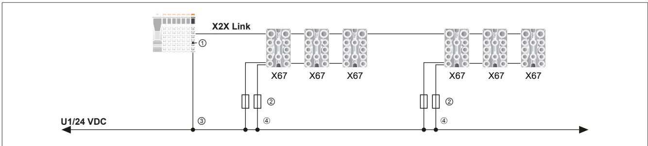
Figure 4: X2X Link cabling - Supply via bus transmitter X20BT9400
