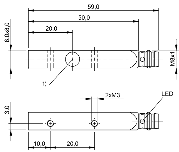
1) Sensing surface
