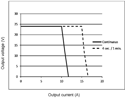
Load lines
