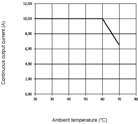
Load lines
