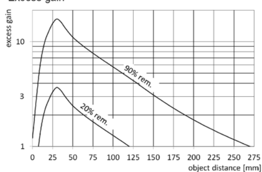
Excess gain
