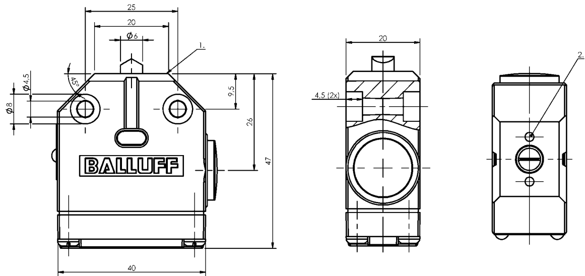
1) Reference edge, 2) Mark. Safety switch position
