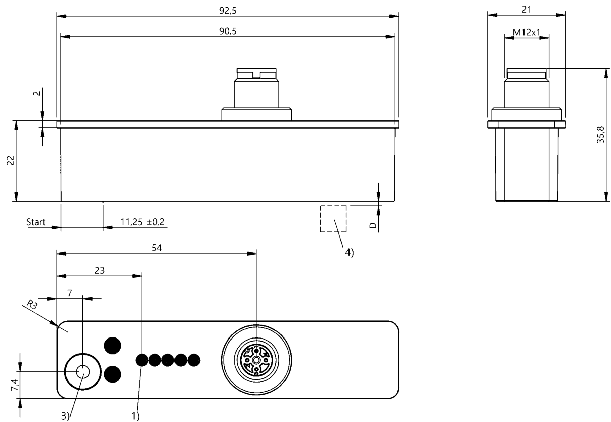
1) LED function indicator, 3) Teach-In button, 4) Encoder
