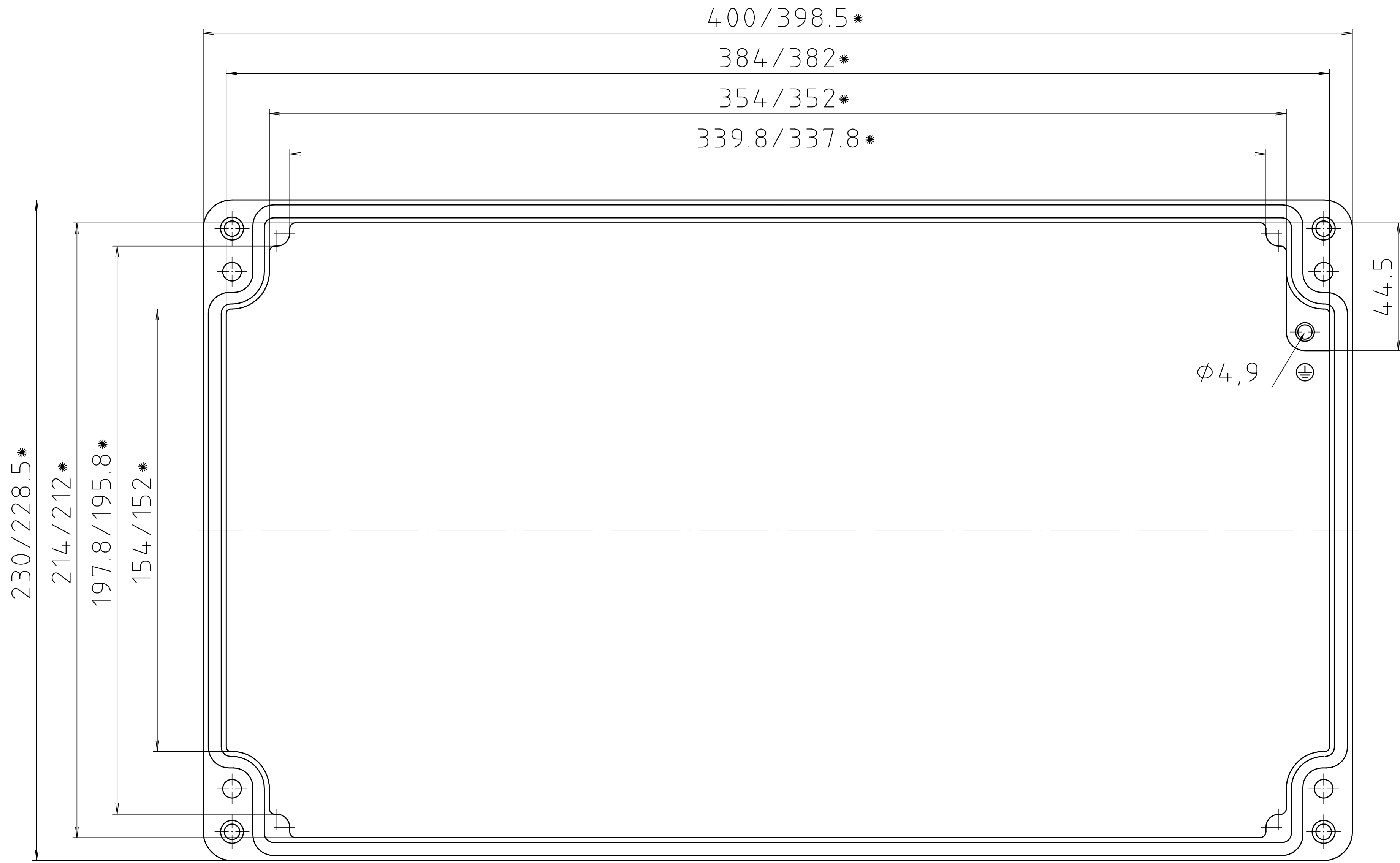
Deckel/lid
