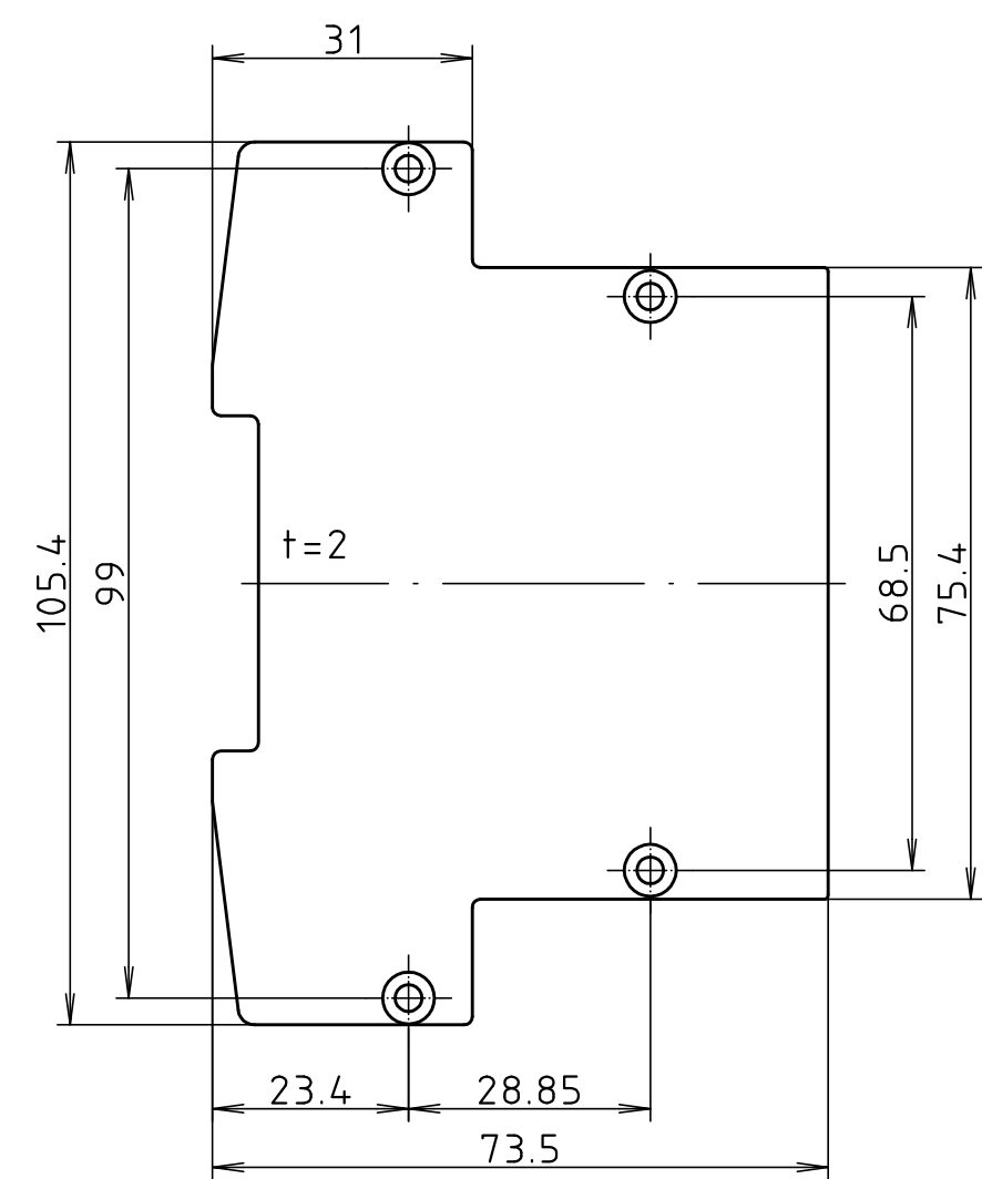
AR 105/75-KS-AL
