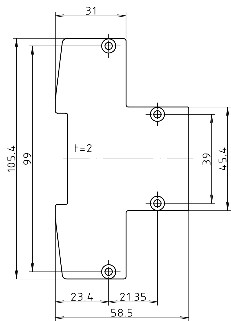
AR 105/45-KS-AL
