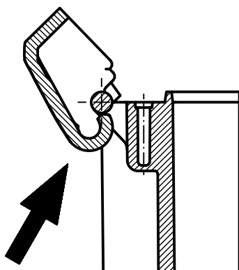
B SC 13 Montagerichtung B SC 13 mounting direction
