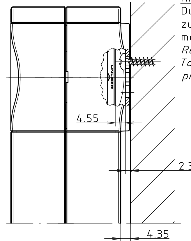
Wandmontage / Wall mounting
