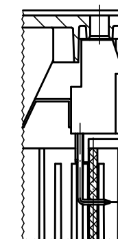
Anschlussklemme AK 700/. HB/ Connection terminals AK 700/. HB
