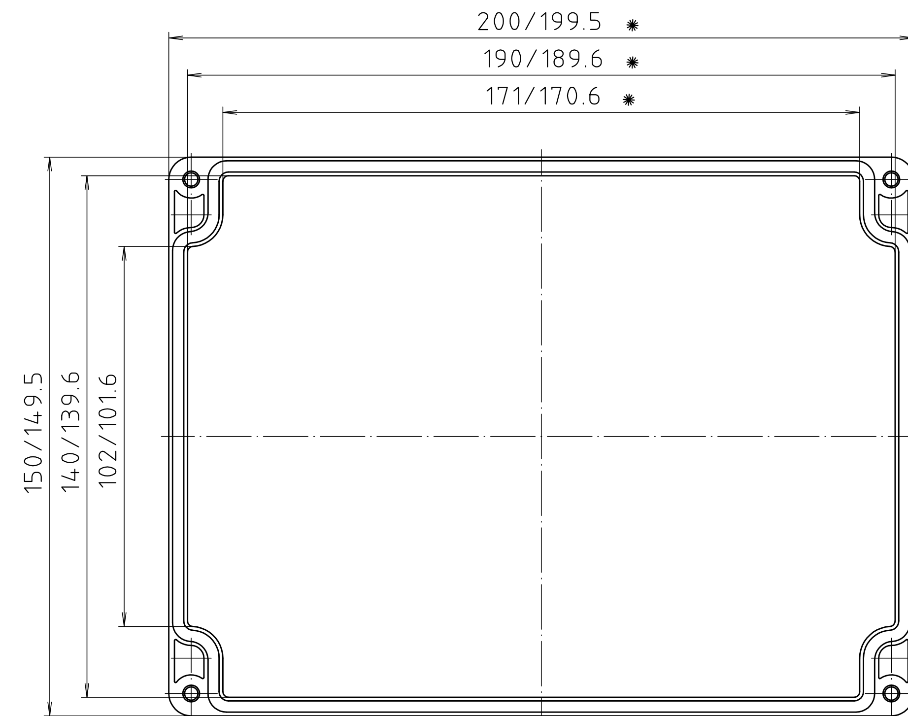
Deckel/lid
