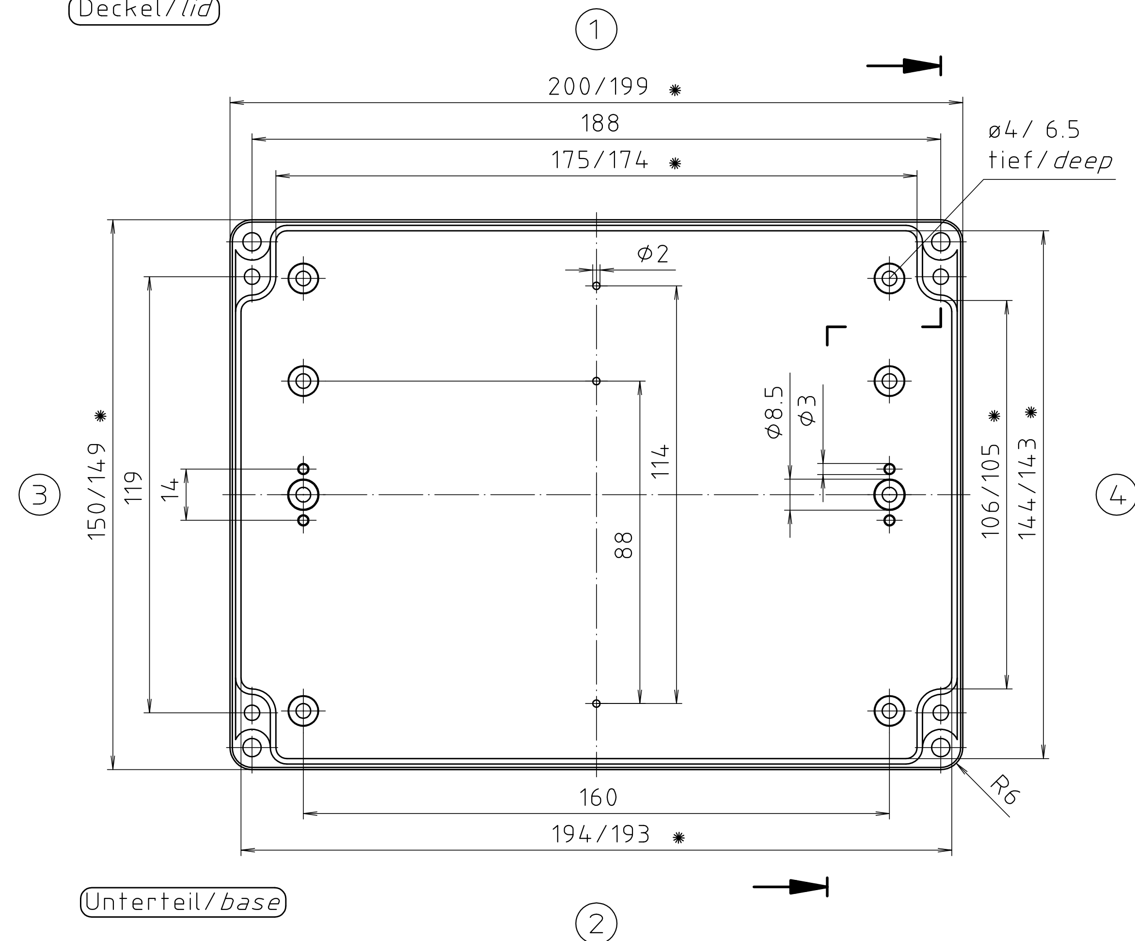
Deckel/lid
