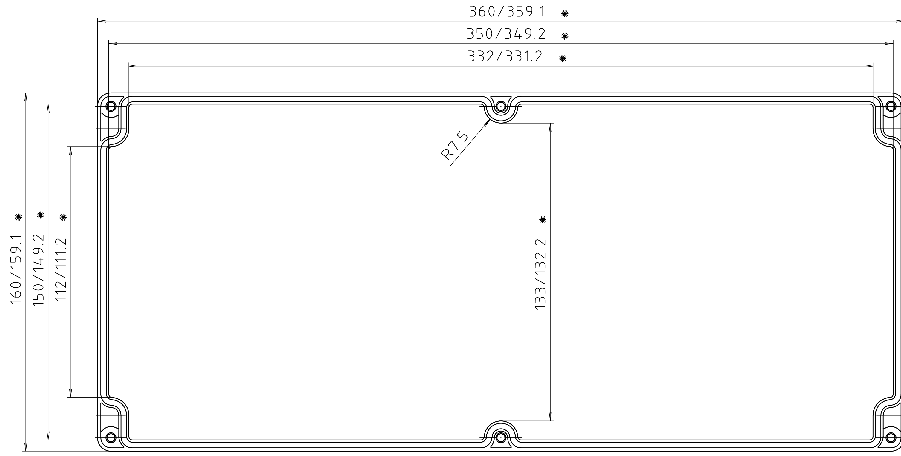
Deckel/lid
