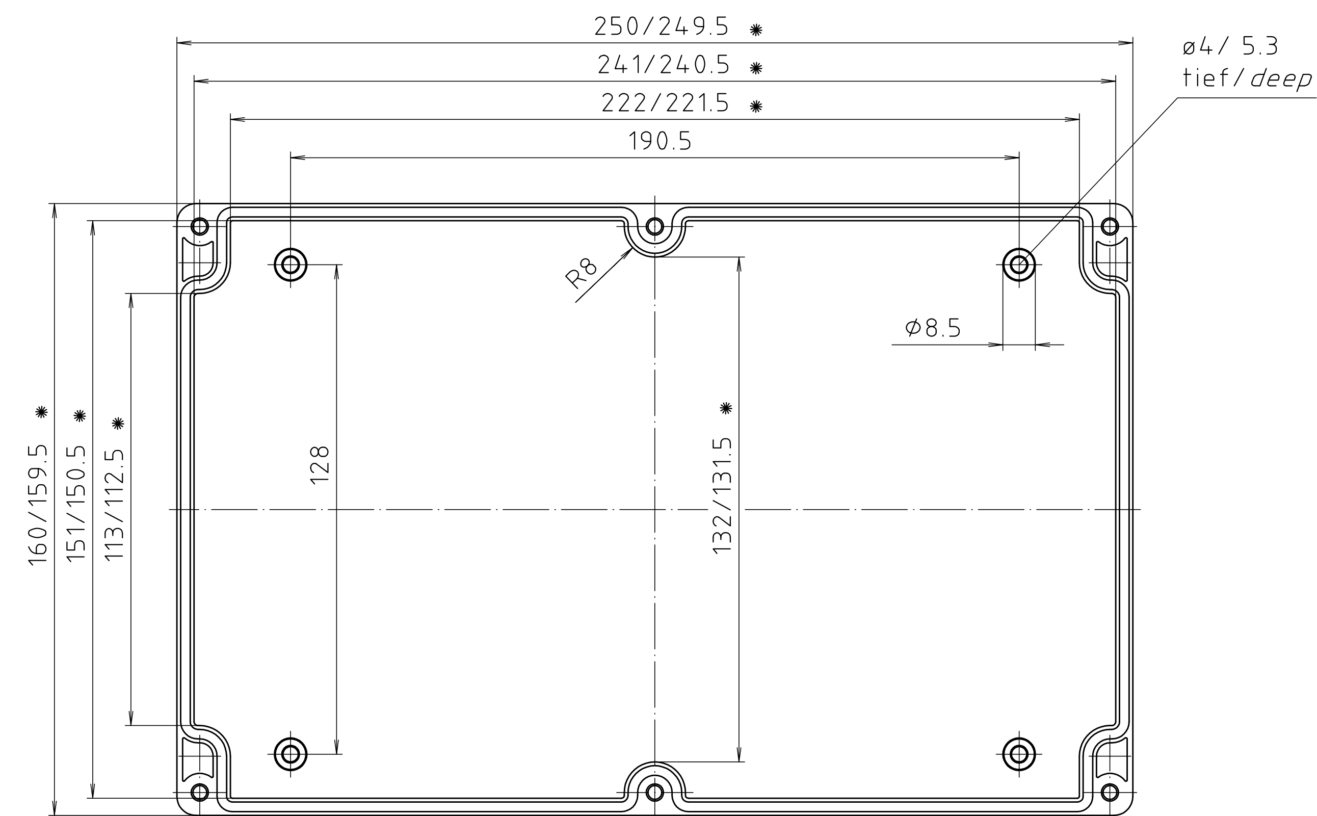
Deckel/lid
