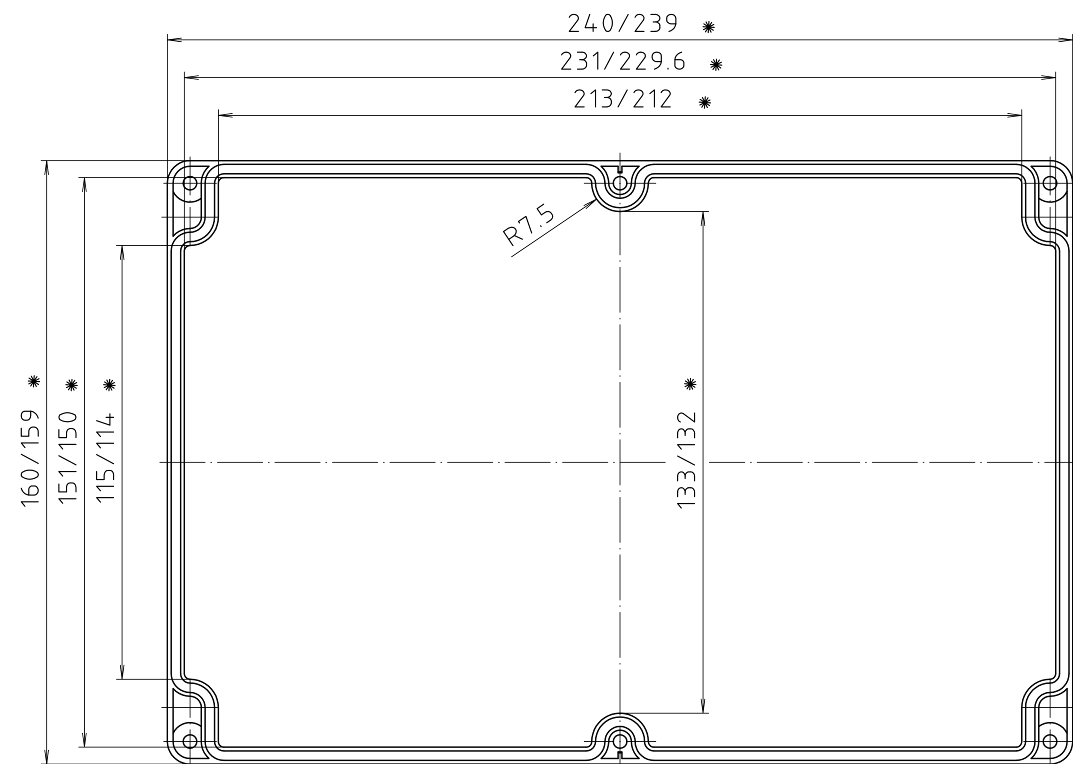
Deckel/lid
