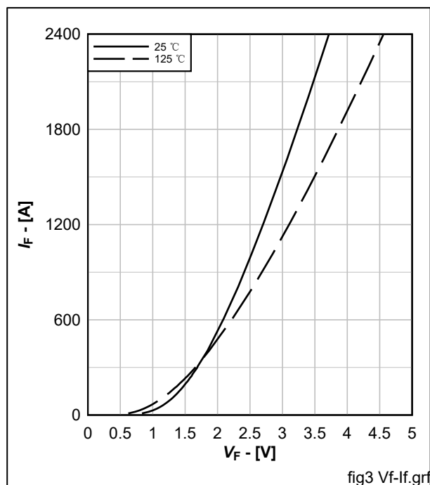
Fig.3 Typical output characteristics, I_F = f(V_F)
