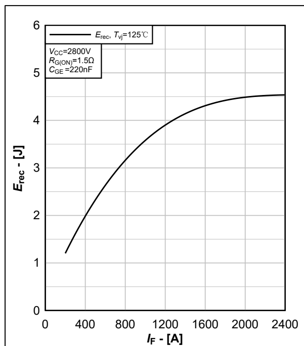
Fig.4 Typical reverse recovery energy, E_{rec} = f(I_F)
