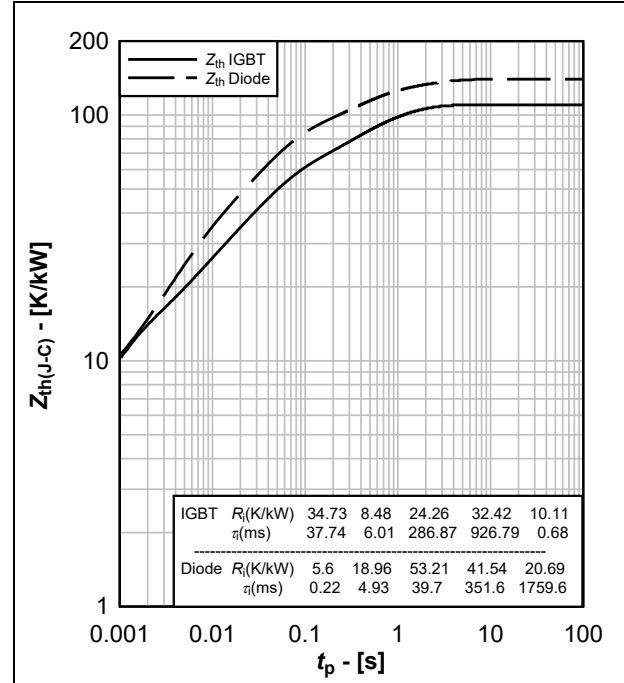
图 16. 瞬态热阻抗曲线, Z_{th(U-F)} = f(t_p)
