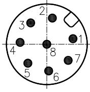
Male(Front view)
