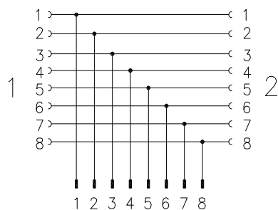
Circuit diagram:
