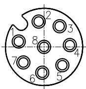
Female(Front view)
