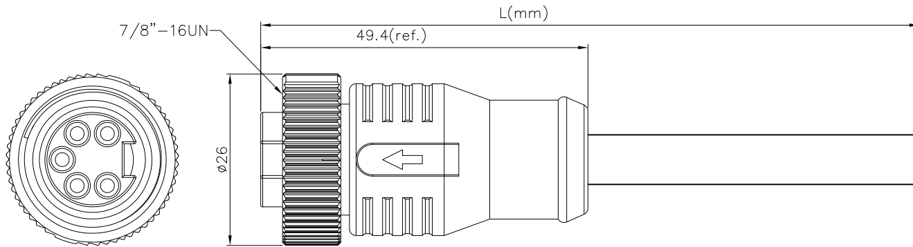
Conn1
