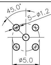
PCB Layout
