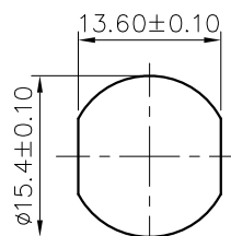
Panel Mounted
