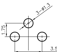
PCB layout
