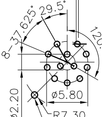
PCB Layout
