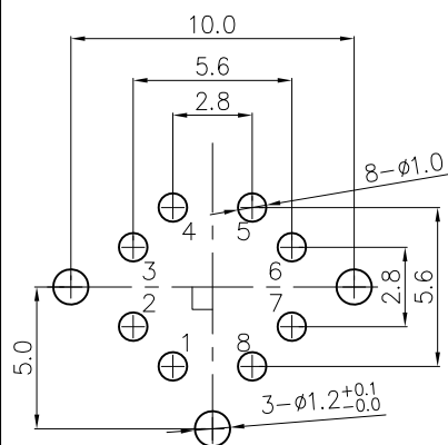
PCB Layout
