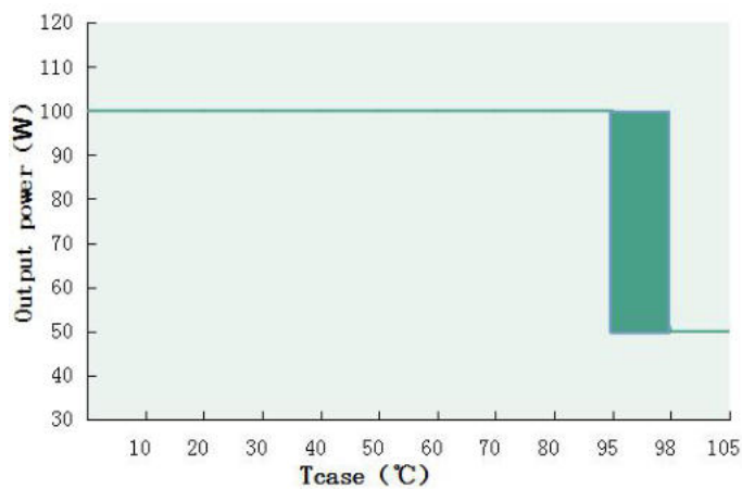
Output power VS Tcase (DL-100H-MAL)
