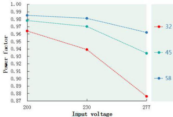
Power factor VS Input voltage(DL-100H-MAL)
