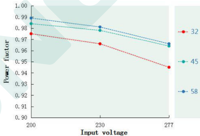
Power factor VS Input voltage(DL-100I-V58P/A-MAS)
