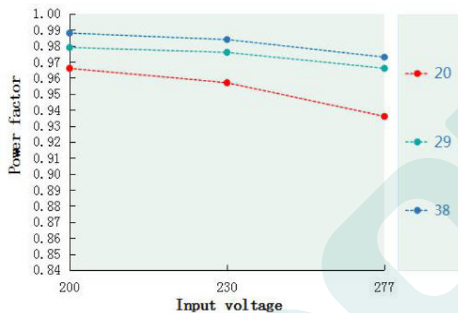
Power factor VS Input voltage(DL-100I-V38P/A-MAS)
