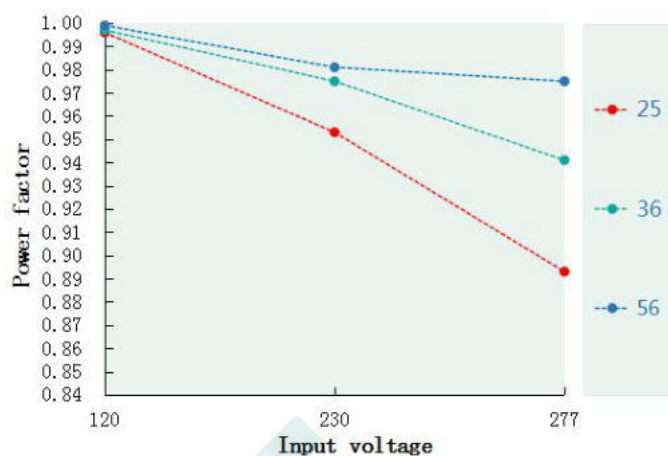
Power factor VS Input voltage(DL-100W-V56A/P/X-MDK)
