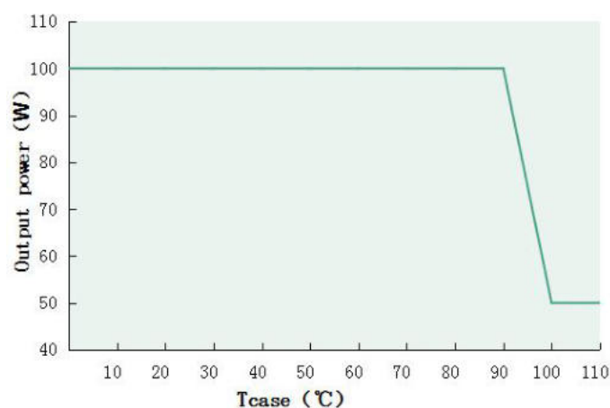
Output power VS Tcase (DL-100W-A/P/X-MDK)
