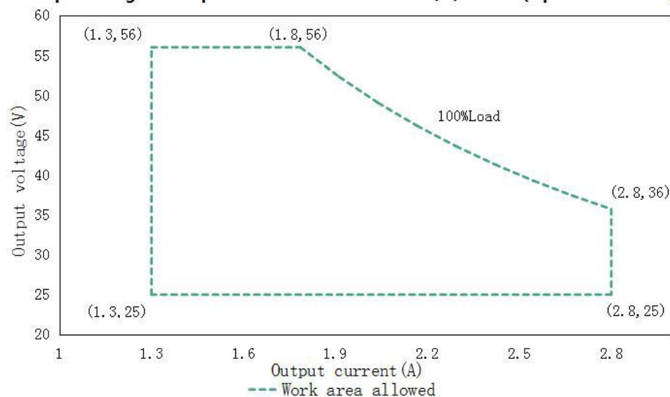
Output voltage VS output current of DL-100W-V56A/P/X-MXG (input: 120-277Vac)
