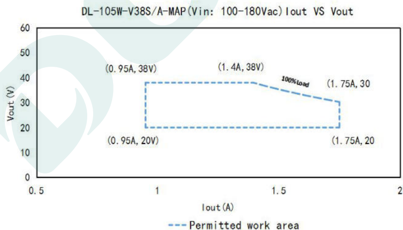
DL-105W-V38S/A-MAP(100-180Vac , Rated output current and output power corresponding to different load voltages)
