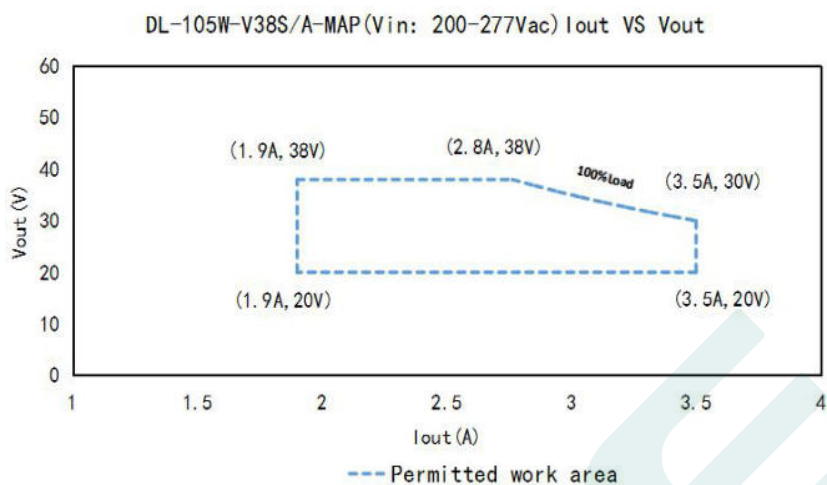
DL-105W-V38S/A-MAP(200-277Vac , Rated output current and output power corresponding to different load voltages)
