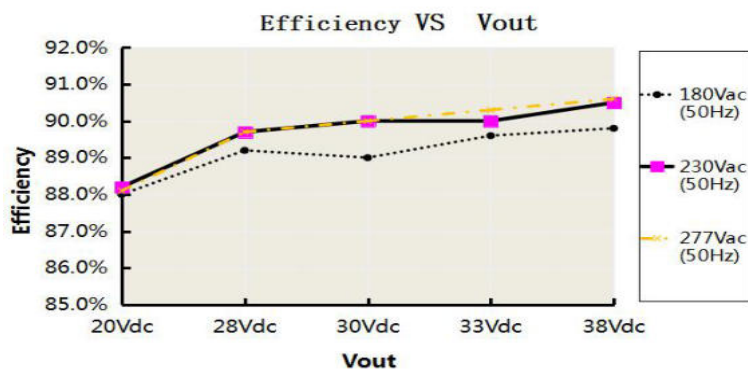
■ Efficiency VS Vout(DL-105W-V38S-MAP)
