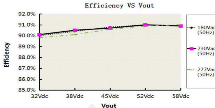
■ Efficiency VS Vout(DL-105W-V58S-MAP)
