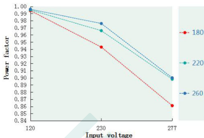
Power factor VS Input (DL-120W-V260A/S/X -SPF)
