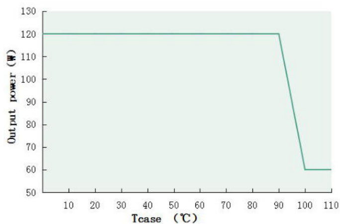
Output power VS Tcase (DL-120W-V260A/S/X -SPF)
