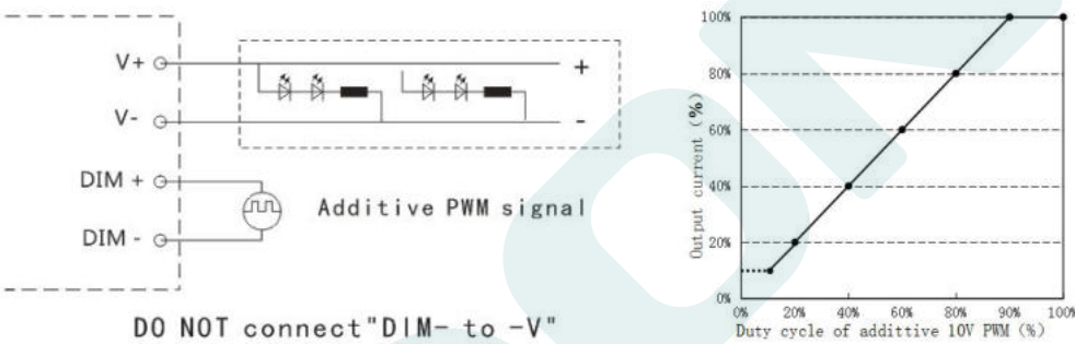
dimming curve
