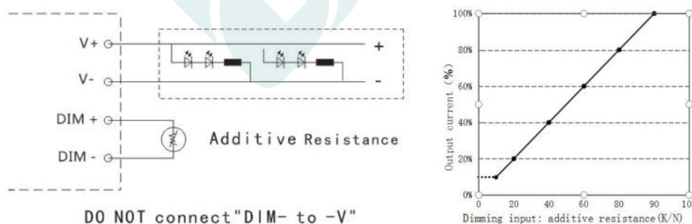
dimming curve
