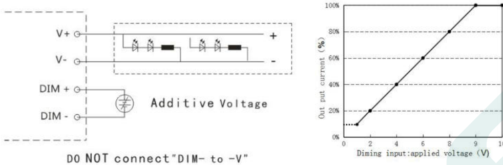
dimming curve
