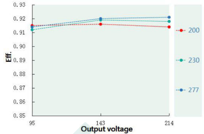
Eff. VS Output voltage DL-150H-214P/A-MXC
