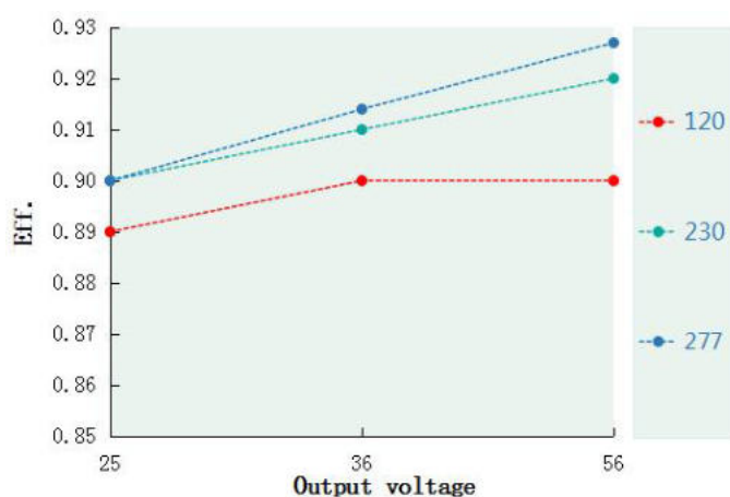
Eff. VS Output voltage(DL-150WK-V56A/P-MXG)
