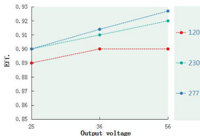
Eff. VS Output voltage(DL-150WK-V214A/P-MXG)
