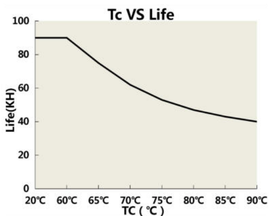
■ Tc VS Life (DL-150W-S/A-MAP)
