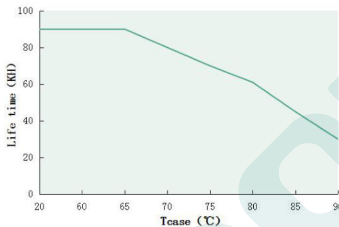
Tcase VS Lifetime(DL-150H-V38P/A-MAS)
