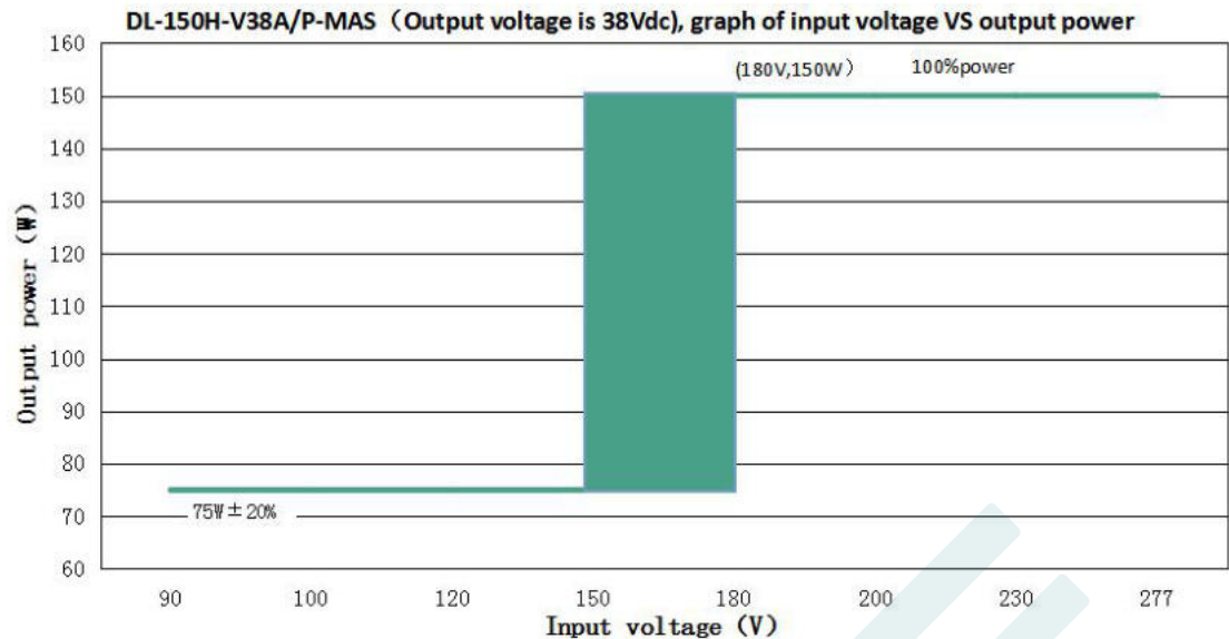
DL-150H-V38P/A-MAS (For output 38Vdc, the rated output current & power under different input voltage)
