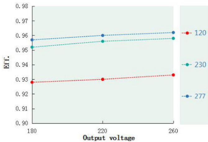
Eff. VS Output voltage(DL-150W-V260A/S/X-SPF)
