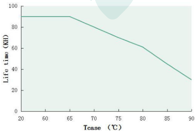
Lifetime VS Tcase (DL-150W-V260A/S/X-SPF)
