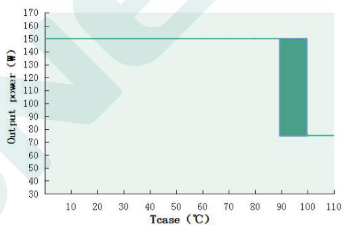
Output power VS Tcase (DL-200H-MAL)
