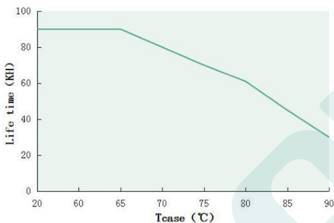
Tcase VS Lifetime(DL-200H-MAL)
