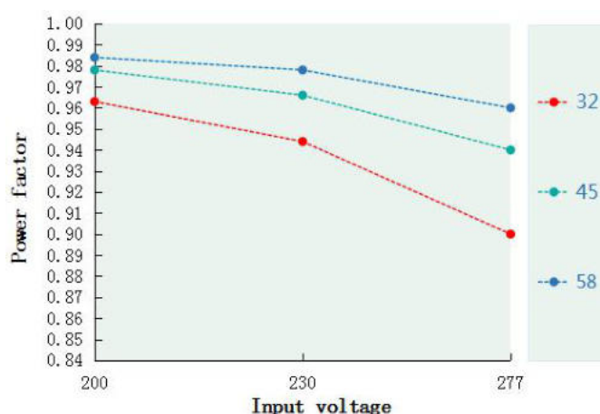
Power factor VS Input voltage(DL-200H-MAL)
