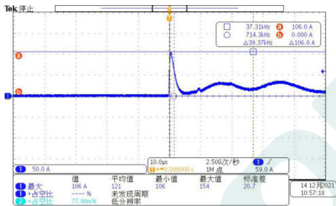
Inrush Current(DL-200I-A/P-MAS)
