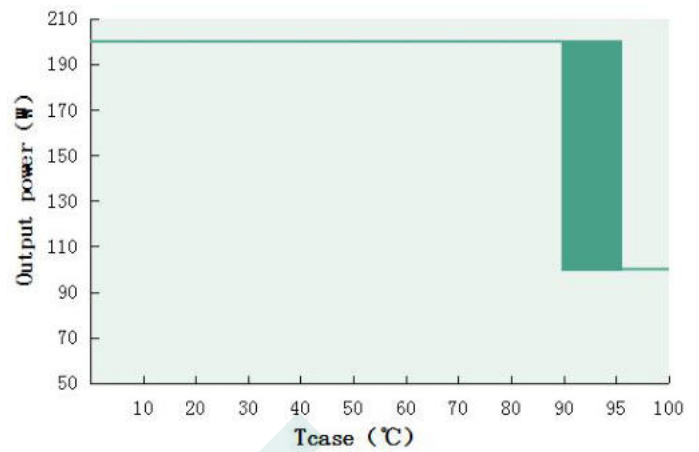
Output power VS Tcase (DL-200I-V58P/A-MAS)
