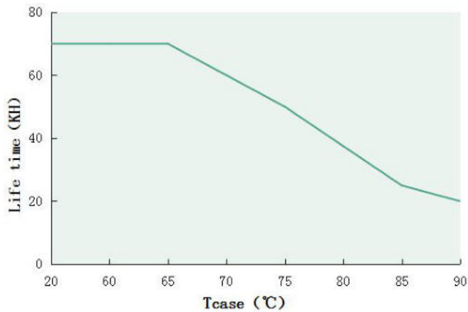
Tcase VS Lifetime(DL-200I-V38P/A-MAS)
